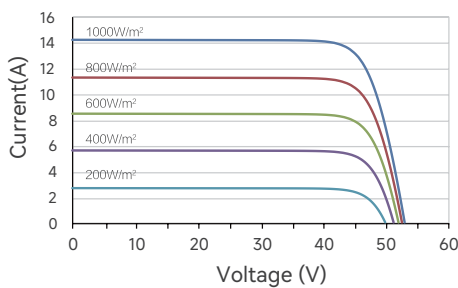
Current-Voltage(600W)
