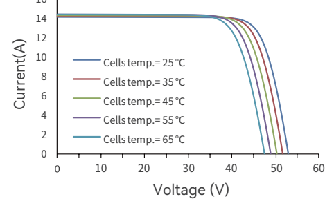
Current-Voltage(600W)
